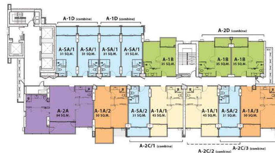
6 th , 7 th , 8 th , 16 th , 17 th , 18 th FLOOR PLAN
